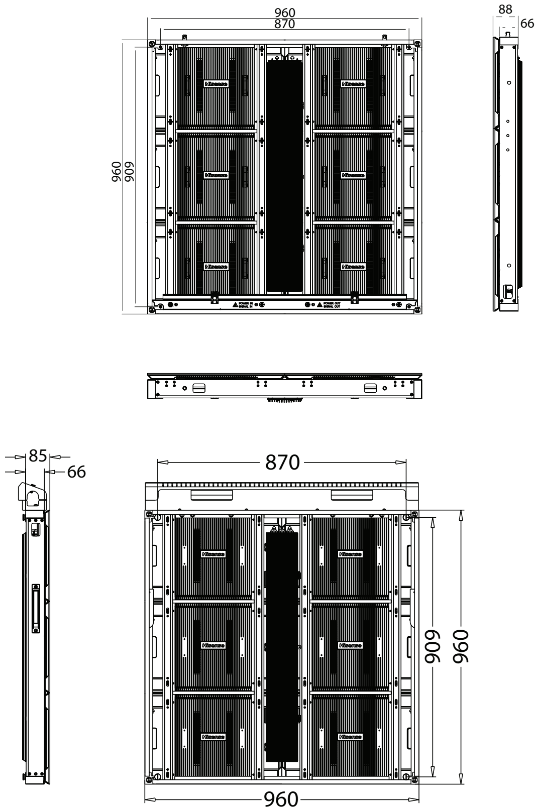
Ribbon Display
