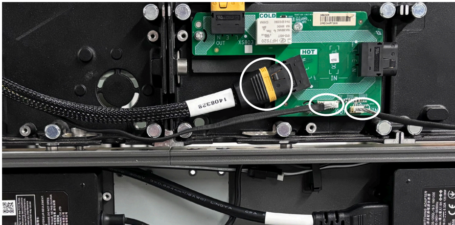
The motherboard cabinet is connected to the schematic diagram
