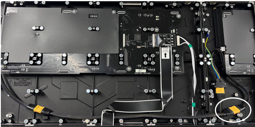
The power cable connection of column 1 to column 2 and column 3 to column 4 for the top line.
