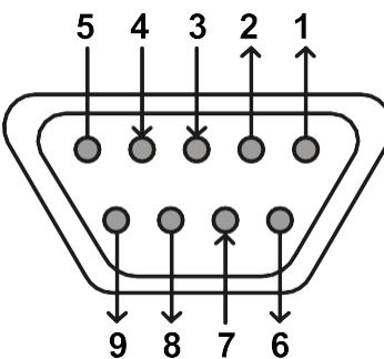
DB-9 Female
