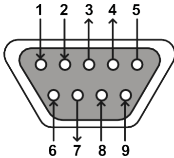
DB-9 Male
