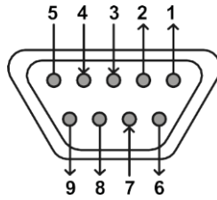
DB-9 Female
